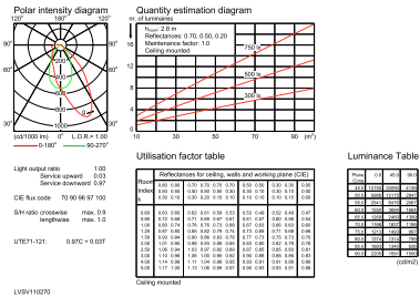
IFGU_4MX900 G3 581 1xLED40S/840 PSU A30-General uniform lighting
