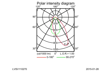
IFPC_4MX900 G3 581 1xLED40S/840 PSU A30-Polar Indoor (combined)
