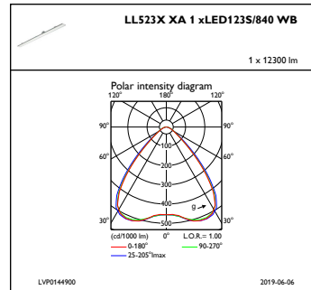
IFPC1_LL523XXA1xLED123S840WB
